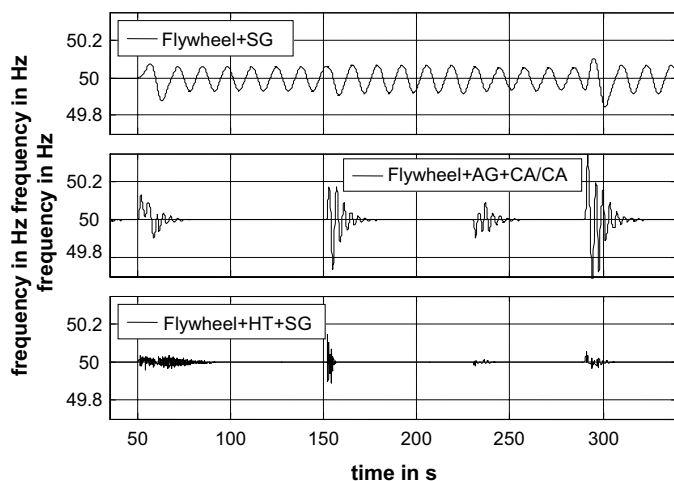
Fig. 11. Frequency in the isolated network.
