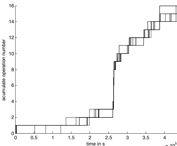
Figure 14 Number of step connection operations in a wind turbine with capacitor steps of the same size.
