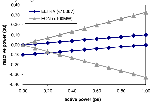
Figure 1 Reactive compensation in ELTRA and EON grid codes
