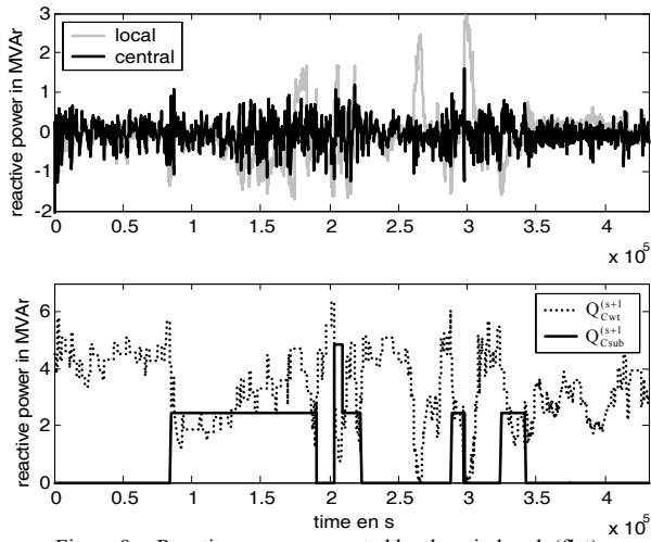
Figure 9 Reactive power generated by the wind park (flat)
