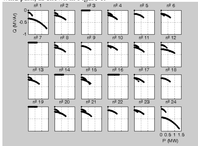
Figure 5 PQ curves from wind turbines
