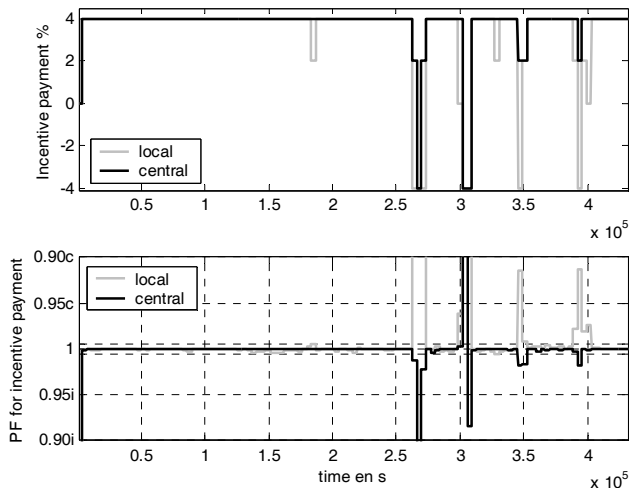
Figure 10 Incentive payment and \cos \phi for each 60 minutes period (flat)
