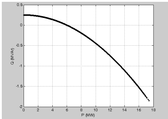
Figure 6 Reactive losses versus the power generated by the wind park
