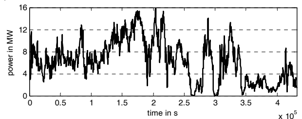
Figure 8 Power generated by the wind park (measured in substation)
