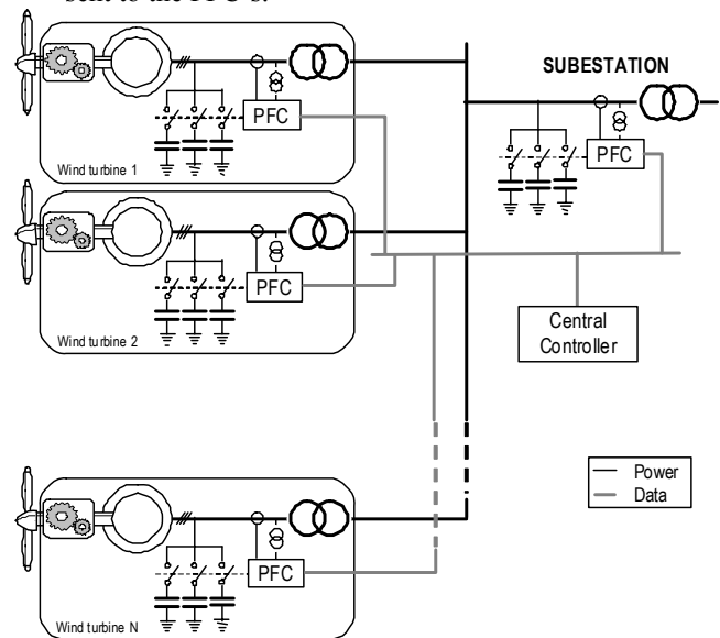
Figure 2 Wind park with a central controller for reactive compensation
