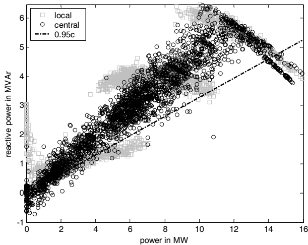
Figure 13 Active power versus reactive power (peak)
