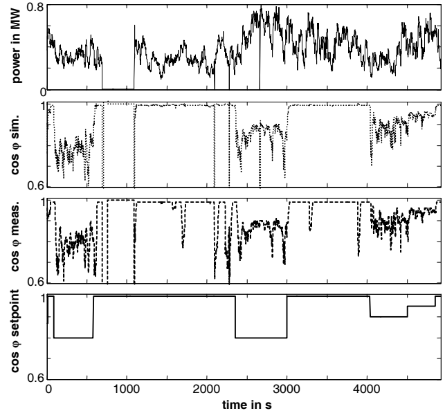
Figure 7 PFC simulation results
