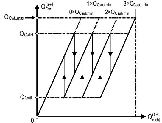
Figure 3 Hysteresis process to allocate the required reactive power between substation and wind turbines
