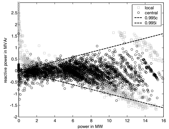
Figure 11 Active power versus reactive power (flat)
