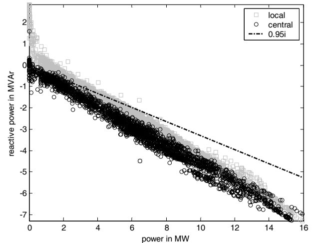
Figure 12 Active power versus reactive power (valley)
